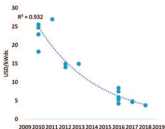
Figure 3: Observed solar O&M costs, 2009-2019 3
