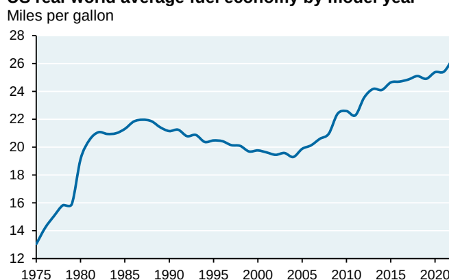
US real-world average fuel economy by model year
