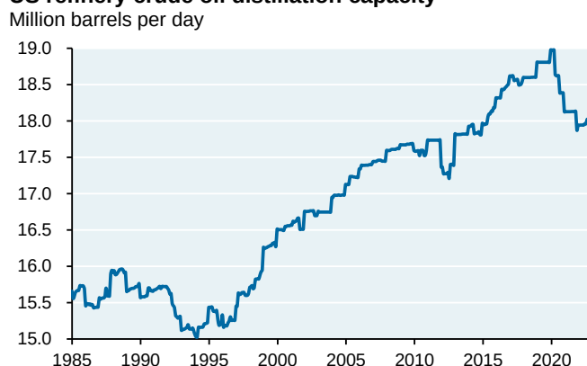
US refinery crude oil distillation capacity
